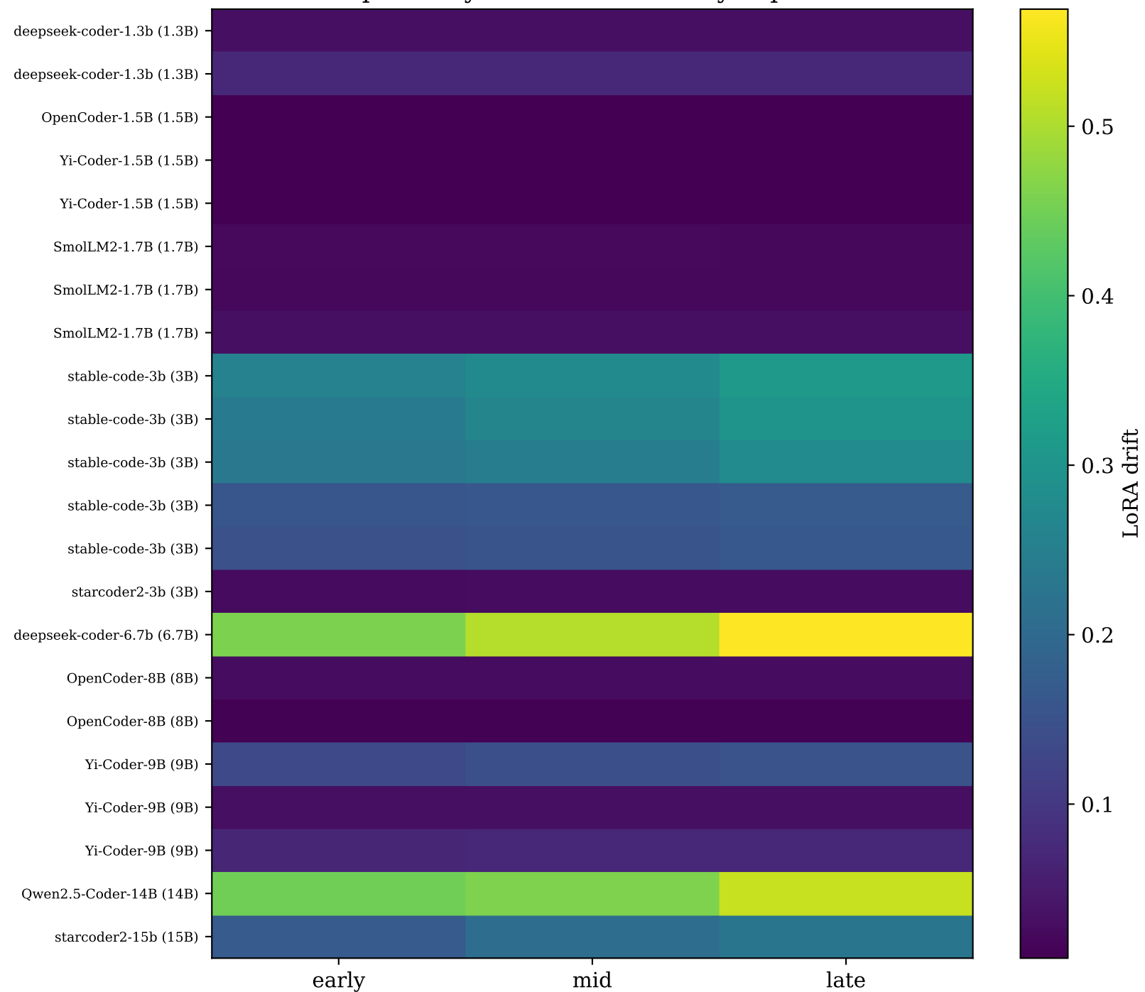
Where plasticity lives: LoRA drift by depth \times scale
