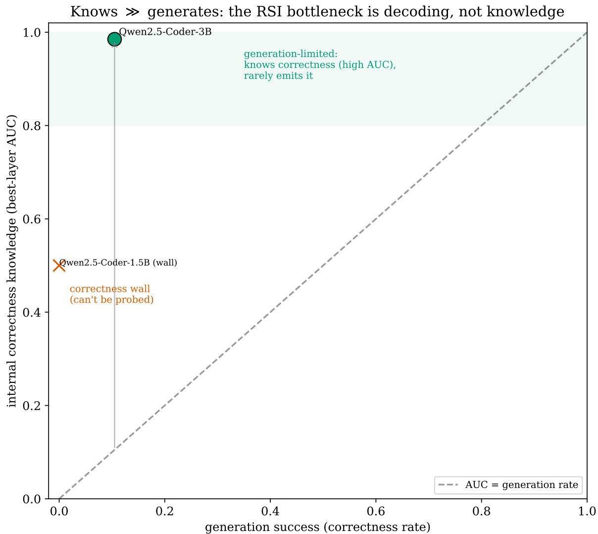
Figure 24: Internal correctness knowledge (best-layer probe AUC) vs. actual generation success. Points far above the diagonal are generation-limited – the model represents correctness internally ( \text{AUC} \approx 0.98 ) yet emits a correct kernel only a small fraction of the time; models at the wall cannot be probed at all.
