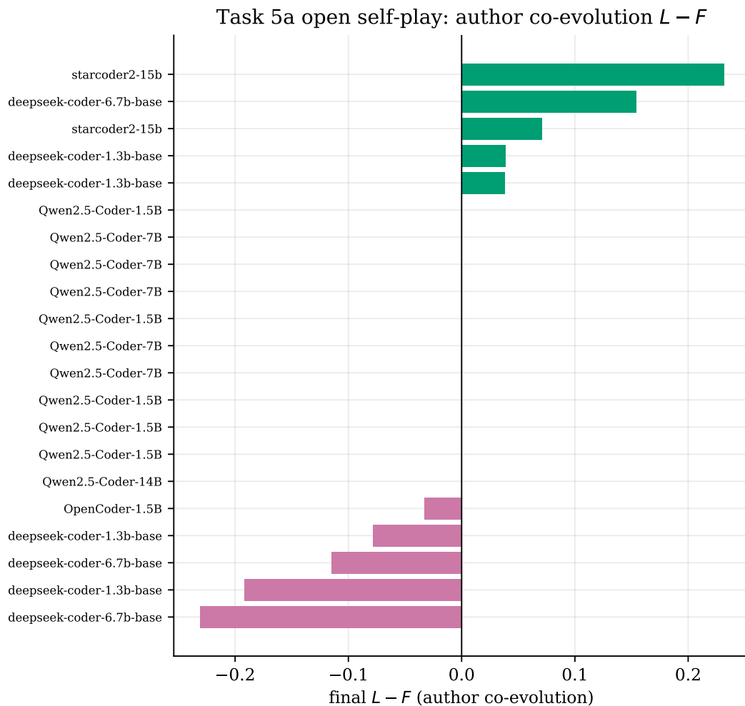
Figure 6: Final L - F (live-author minus frozen-author, the self-referential signal) per open-weight model. > 0 means updating the author beyond a frozen-author escalating curriculum genuinely helps.
