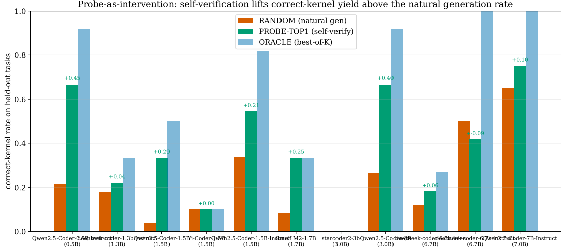
Figure 40: Self-verification (probe-guided selection) vs. the model’s natural single-draw success (RANDOM) and the ORACLE best-of- K upper bound, at equal generation budget K , on held-out tasks. Annotated +\text{lift} = \text{PROBE-TOP1} - \text{RANDOM} . Probe selection recovering much of the oracle gap turns the correlational correctness-AUC into a causal decode-time intervention.
