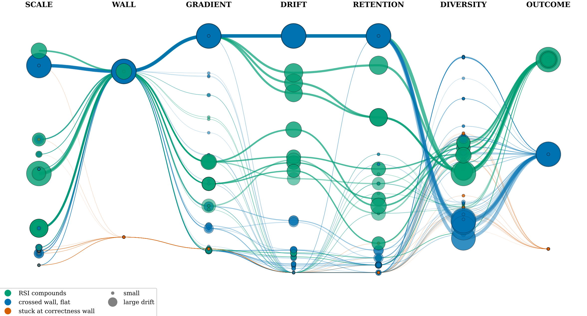
Internal-failure causality DAG: each model's path Scale → Wall → Gradient → Drift → Retention → Diversity → Outcome (133 models; edge width & marker area ∝ LoRA drift)
