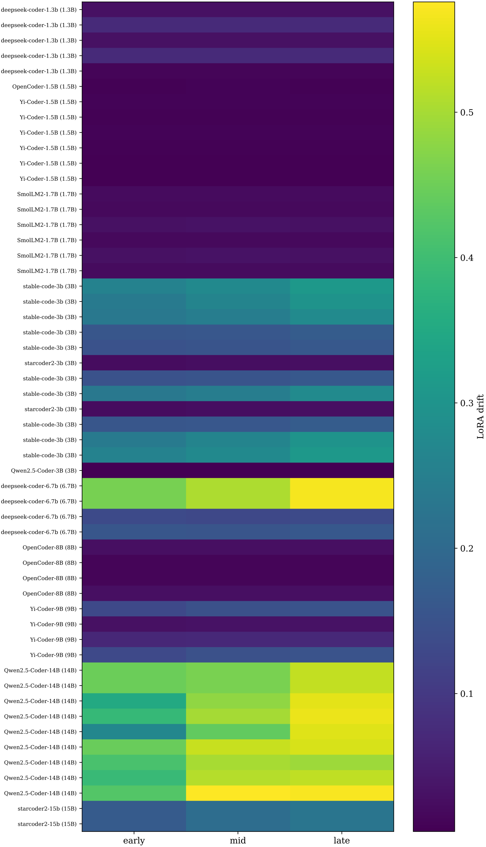
Where plasticity lives: LoRA drift by depth × scale
