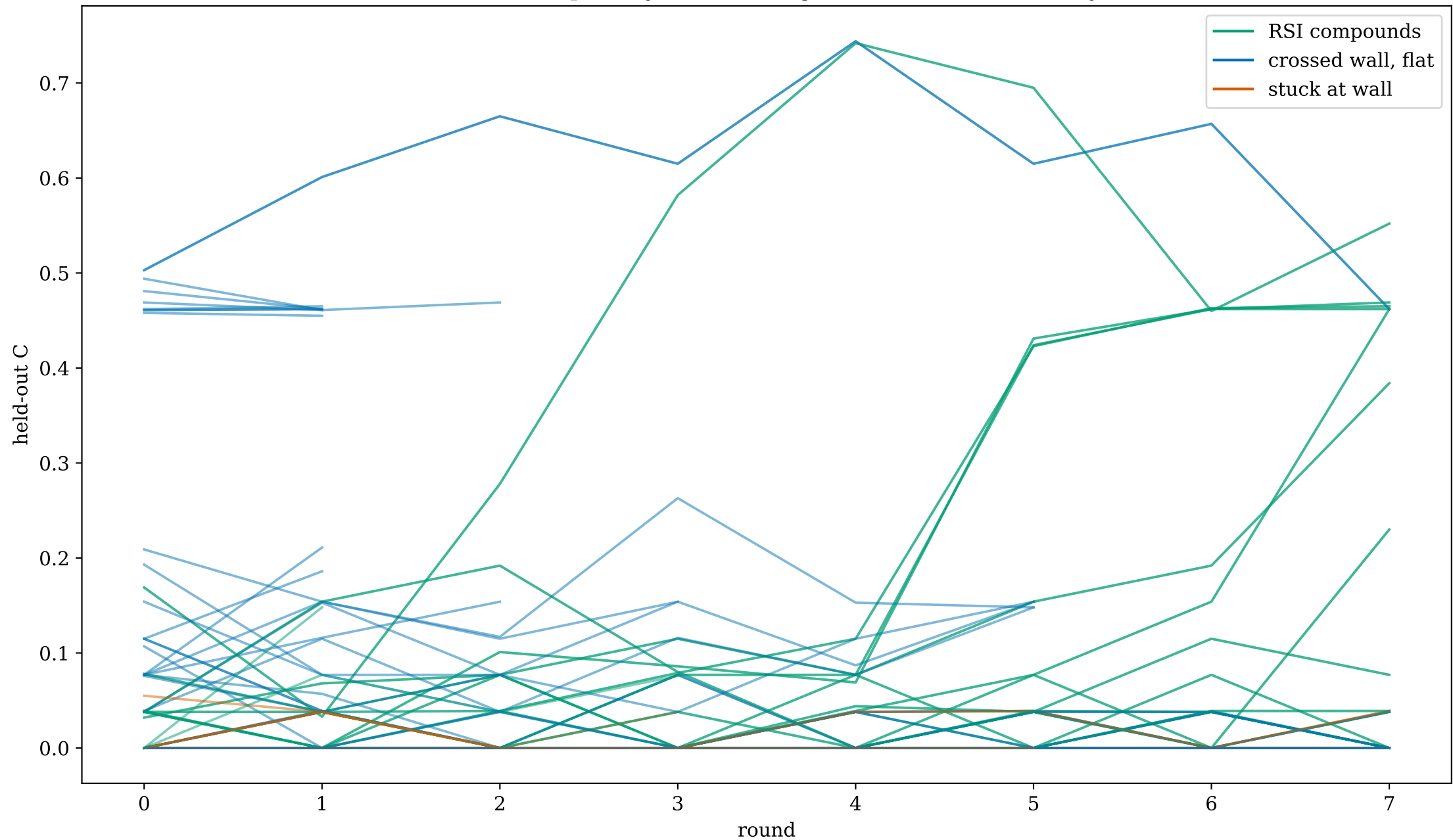
Per-round held-out capability, all 133 weight-RSI runs (coloured by outcome)
