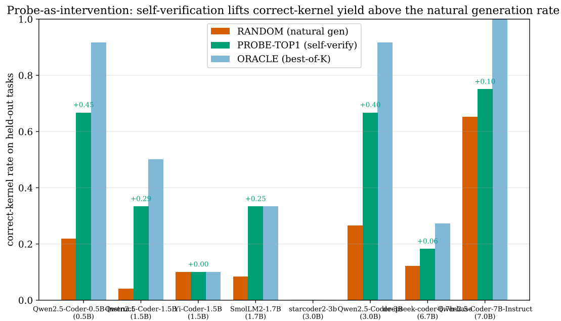
Figure 40: Self-verification (probe-guided selection) vs. the model’s natural single-draw success (RANDOM) and the ORACLE best-of- K upper bound, at equal generation budget K , on held-out tasks. Annotated \text{+lift} = \text{PROBE-TOP1} - \text{RANDOM} . Probe selection recovering much of the oracle gap turns the correlational correctness-AUC into a causal decode-time intervention.
