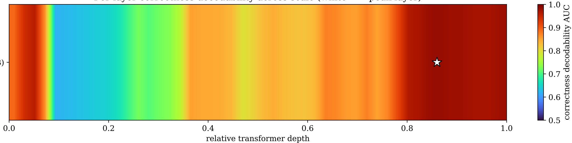
Per-layer correctness decodability across scale (white ★ = peak layer)
