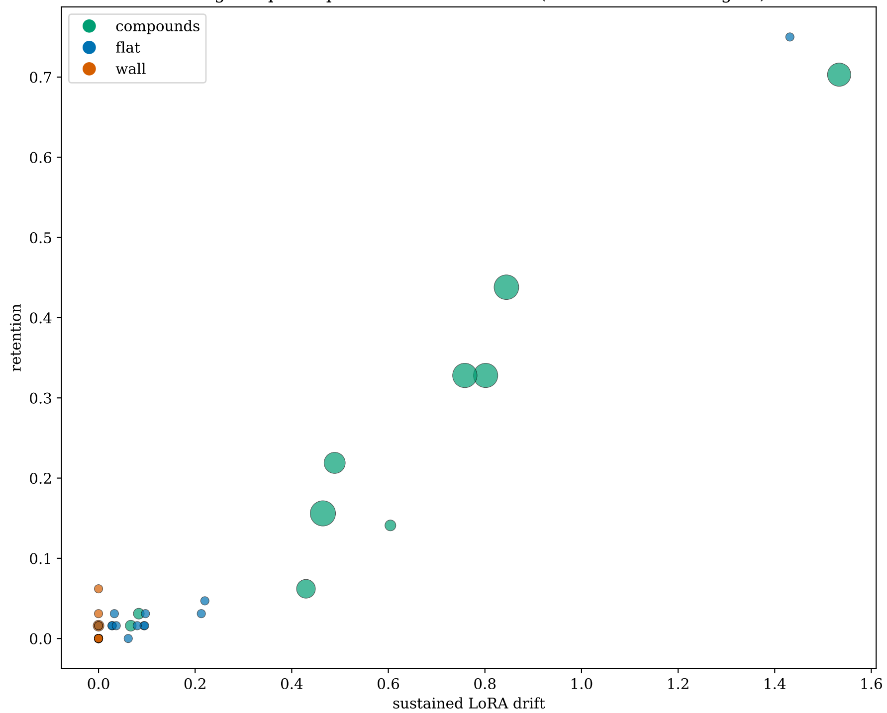
Two-gates phase plane: drift \times retention (marker \propto held-out gain)
