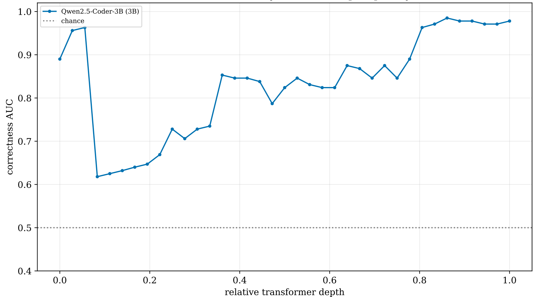
Correctness decodability rises with depth (per-layer)
