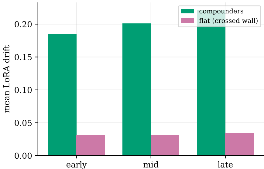
Where learning lives: drift by transformer depth
