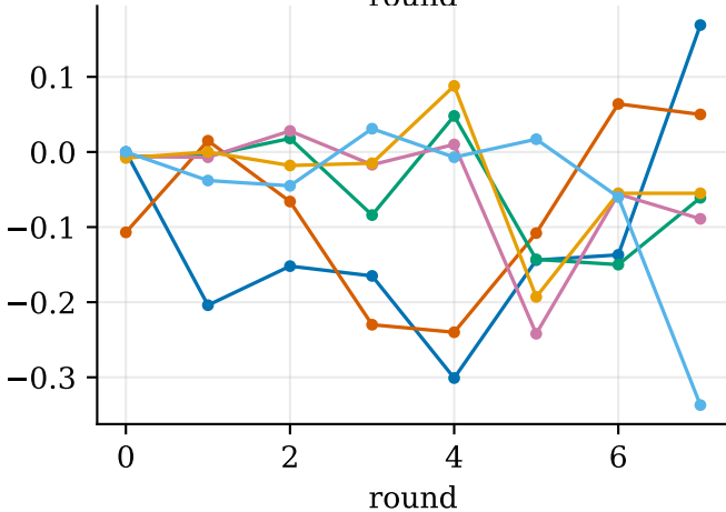
train-held gap
