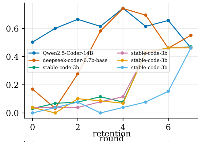
held-out C
