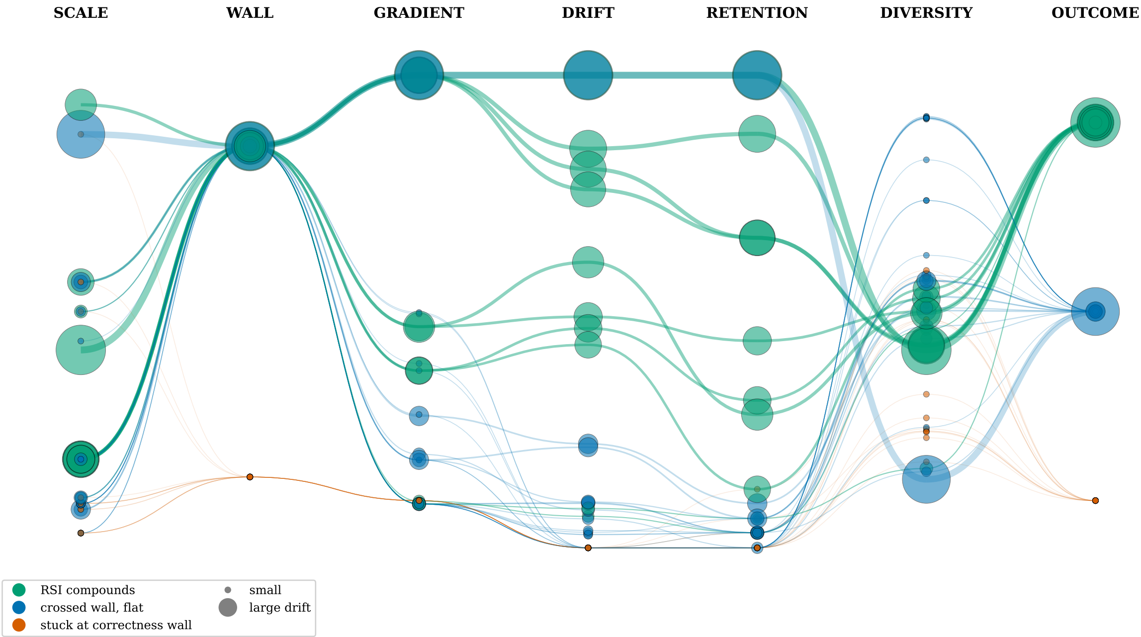
Internal-failure causality DAG: each model's path Scale → Wall → Gradient → Drift → Retention → Diversity → Outcome (50 models; edge width & marker area ∝ LoRA drift)
