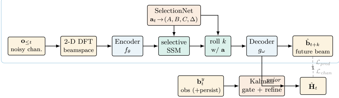
Figure 1: Beam-WM pipeline. The noisy channel history is mapped to the sparse beamspace, encoded, and rolled forward by an action-conditioned selective SSM to predict the future channel ( \mathcal{L}_{\text{pred}} ). The one-step-ahead prediction is a temporal prior that a learned Kalman-style gate fuses with the current noisy observation (and the clean t-1 persistence frame) to estimate the current channel ( \mathcal{L}_{\text{chan}} ). One representation and one backbone serve both tasks.
