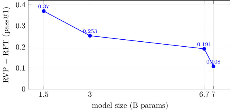
Figure 9: Scale trend (COMPdag-mid). The RVP win shrinks with model size as reliability headroom shrinks, but remains substantial and positive through 7B. At 14B the base is near-ceiling on MATH-500 (.716) and full-parameter DPO OOMs on a single 40 GB device, so 14B falls outside the informative headroom regime rather than extending the trend.
