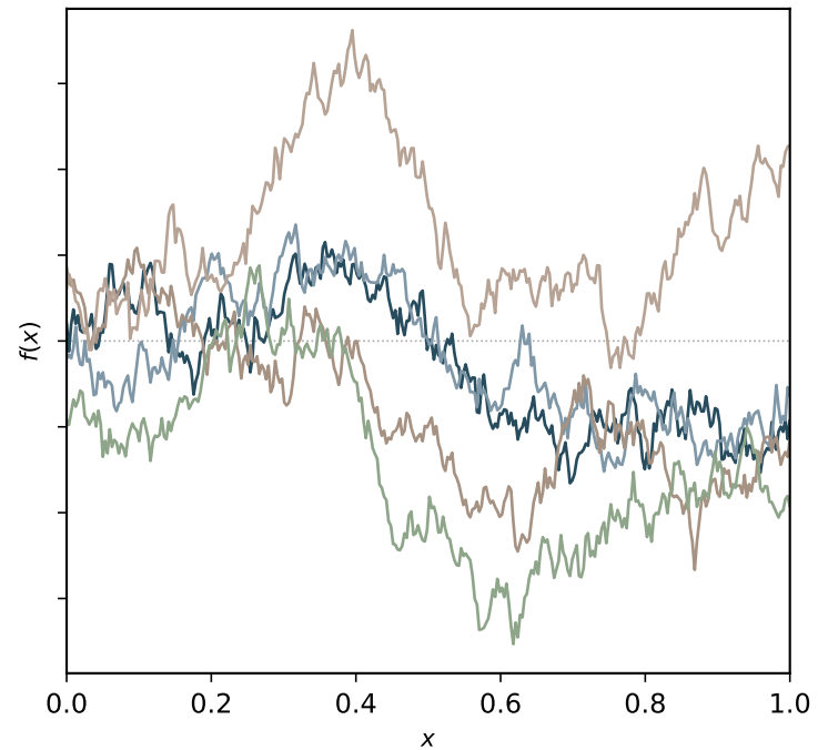
Matern kernel ( \nu = 1/2 )
