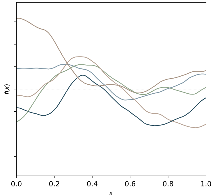
Matern kernel ( \nu = 5/2 )
