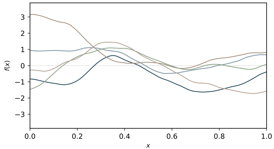
Matern kernel ( \nu = 1/2 )
