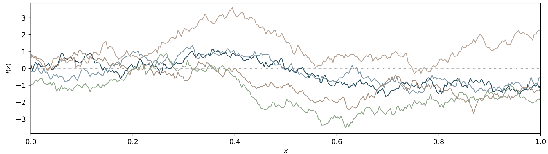
Matern kernel ( \nu = 1/2 )
