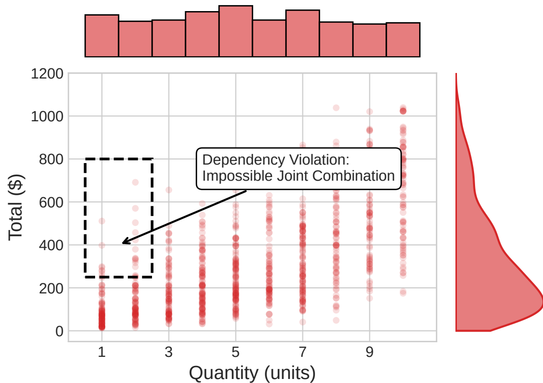
(b) Synthetic Data (Gaussian Copula) (Marginals: KS \geq 0.96 , Joint Violation)
