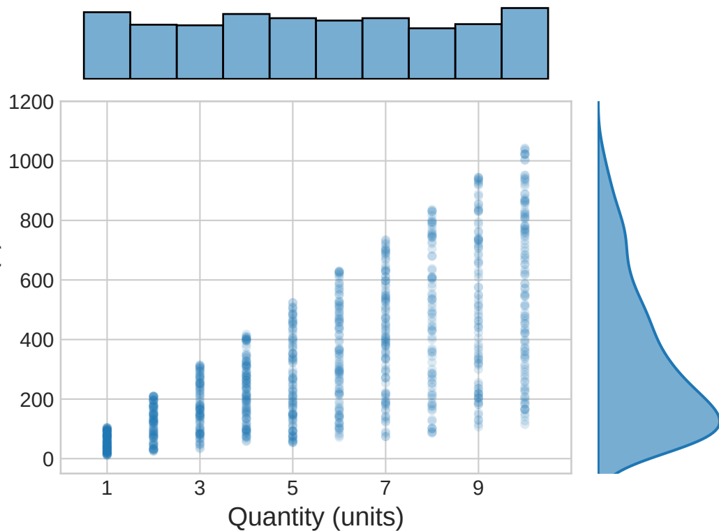
(a) Real Supermarket Data (Ground-Truth Arithmetic Constraint)
