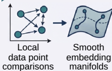
Neighbor-Invariant Continuity
