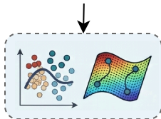
Data Manifold
