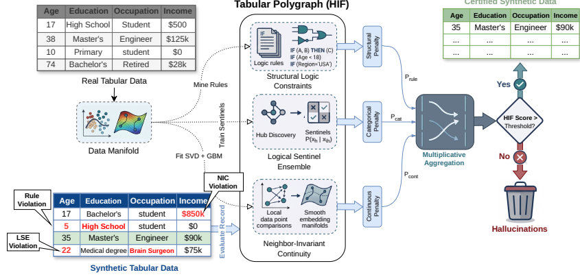
Fig. 2 Architecture of the Hybrid Integrity Framework (HIF). Synthetic tabular data is verified by the Logical Sentinel Ensemble (LSE) and Neighbor-Invariant Continuity (NIC) modules, combined via multiplicative aggregation to filter semantically inconsistent records.
