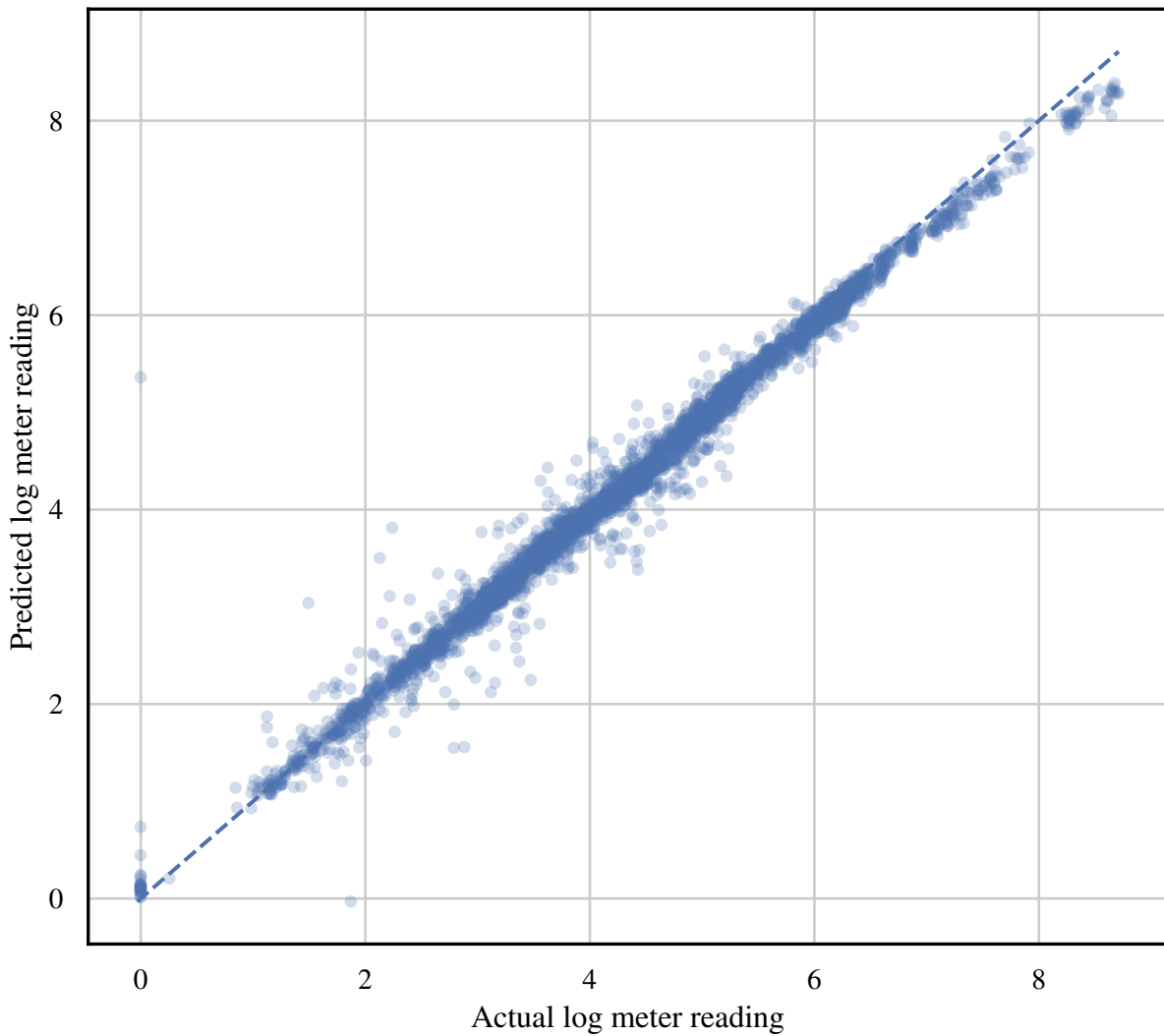
Predicted vs Actual: GRU sequence 24h (best of 5 seeds)
