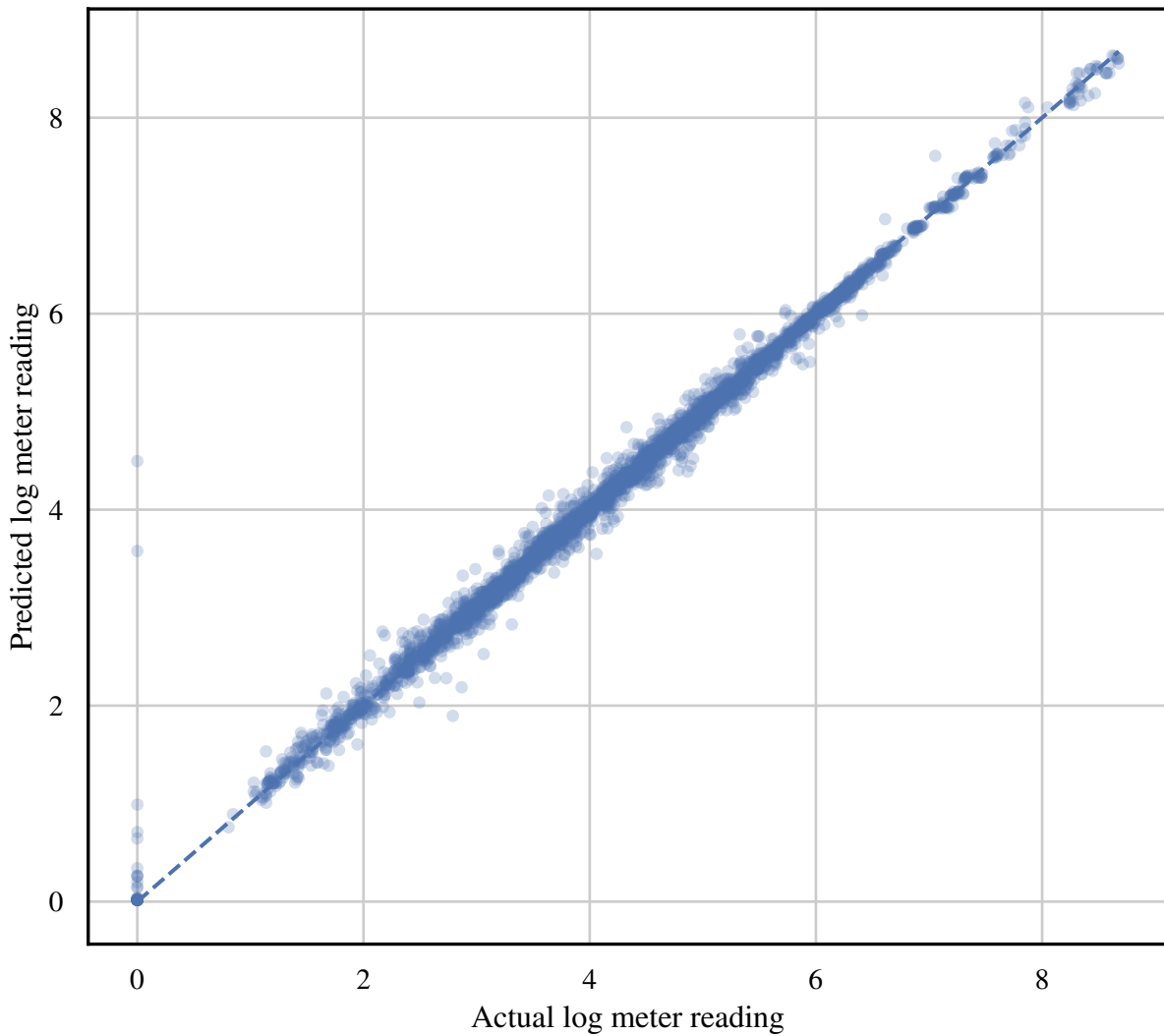
Predicted vs Actual: LightGBM + Lag Features
