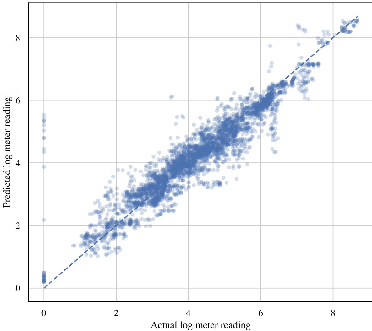
Predicted vs Actual: XGBoost
