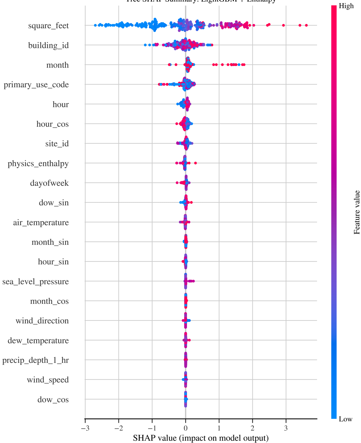
Tree SHAP Summary: LightGBM + Enthalpy
