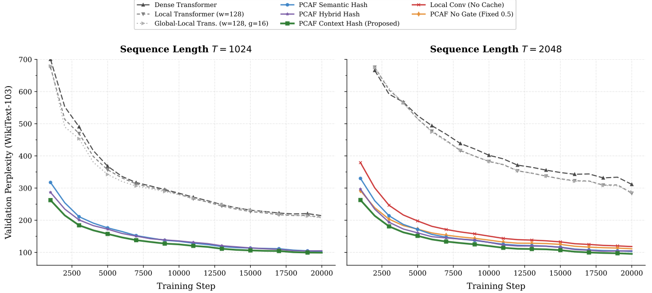
Figure 1: Validation perplexity curves over training steps on WikiText-103 at sequence lengths T = 1024 (left) and T = 2048 (right) on a TPU v4-32 cluster. The proposed pcaf.context routing achieves the lowest perplexity among the evaluated constant-depth associative variants and Transformer baselines.
