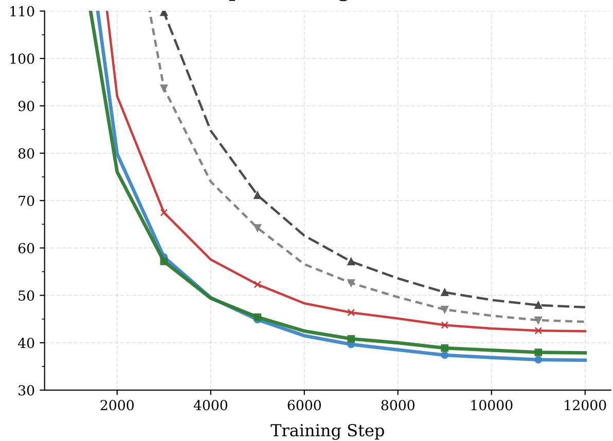
Sequence Length T = 2048
