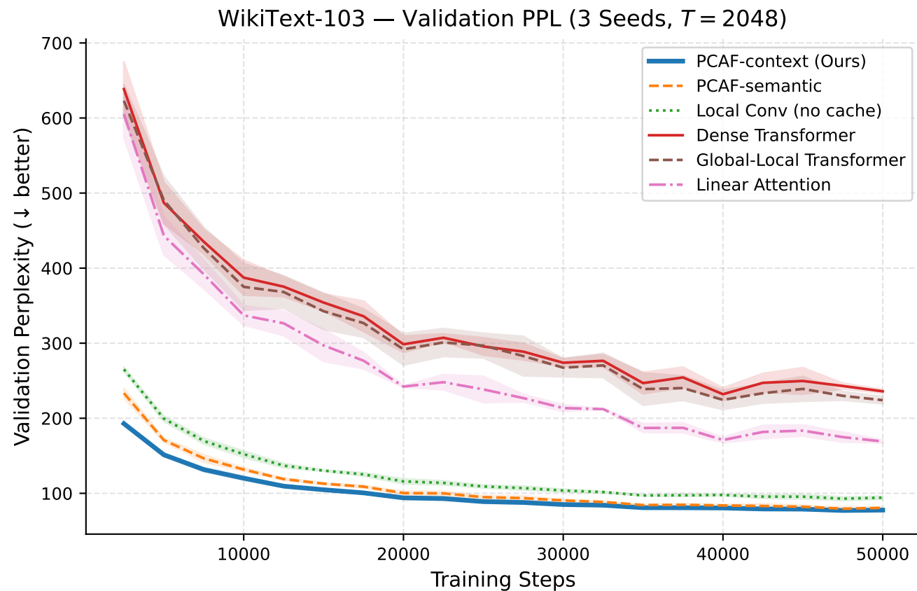
Figure 1: Multi-Seed Validation Perplexity Learning Curves
