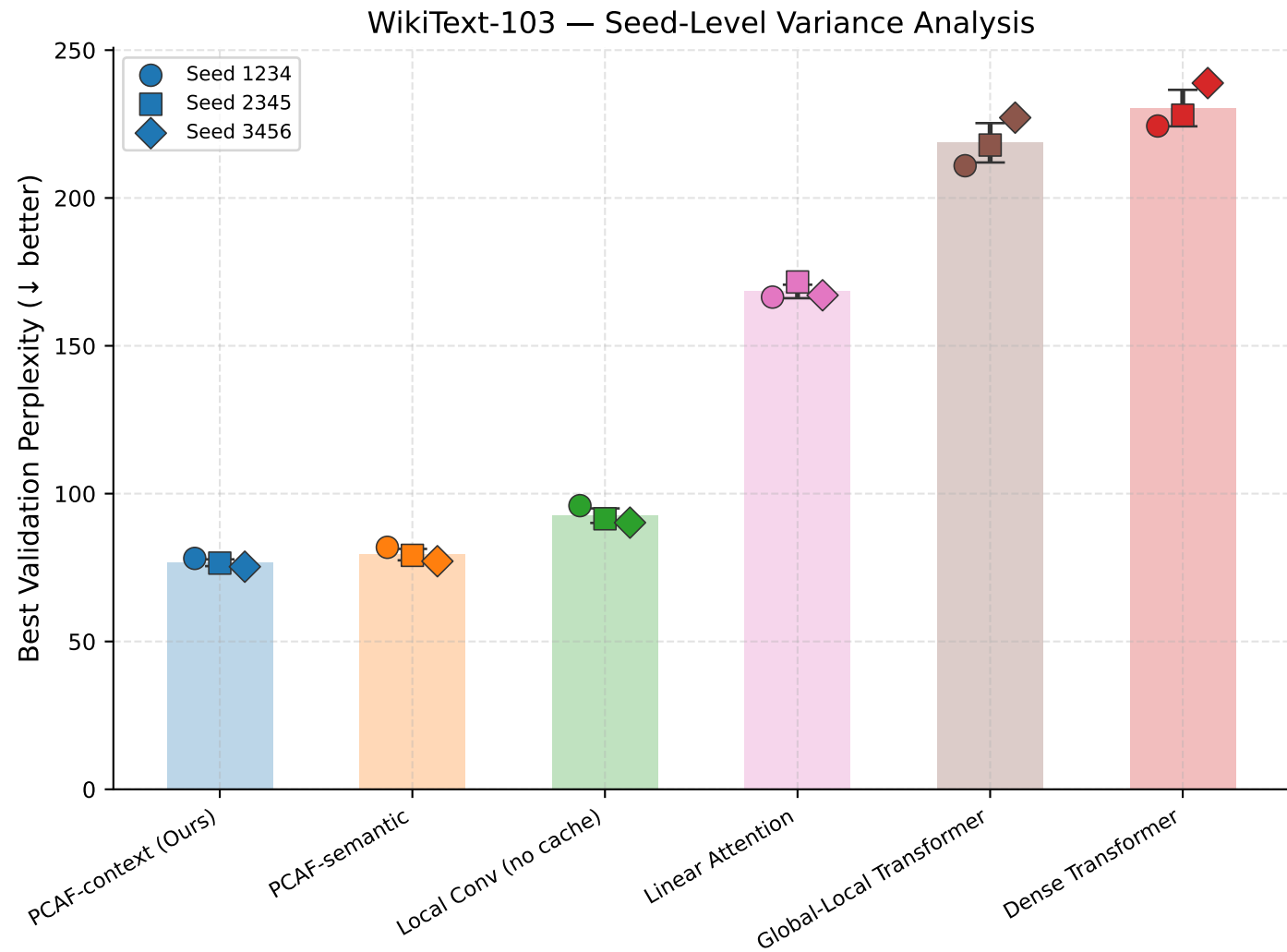
Figure 5: Statistical Robustness — Per-Seed Best Perplexity with Mean \pm Std
