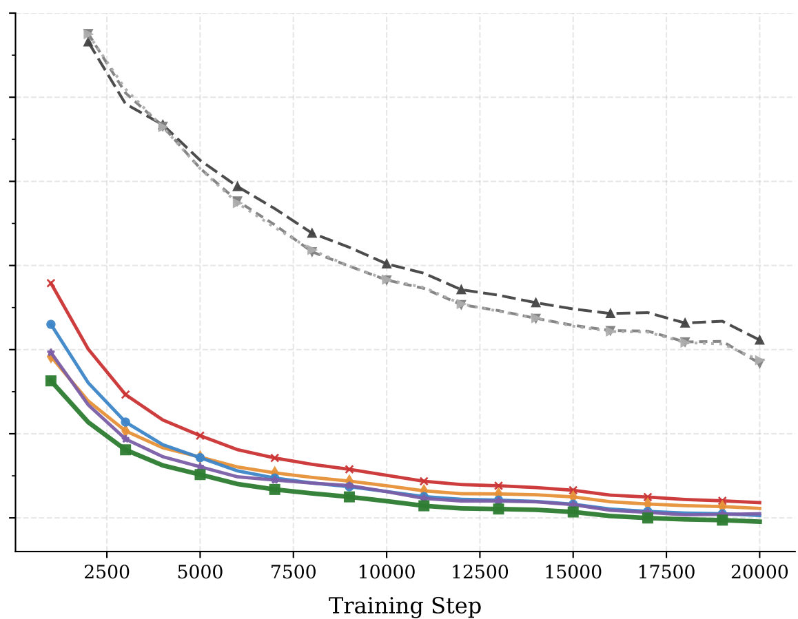
Sequence Length T = 2048
