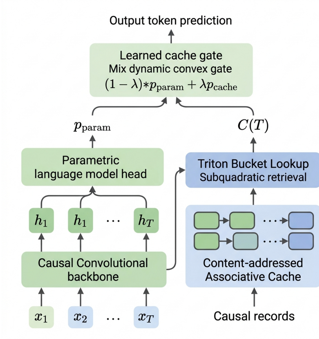
Figure 1: Overall architecture diagram of the proposed Parallel Causal Associative Field (PCAF). Local context is processed via a causal convolutional backbone (bottom) to compute query hidden states, while previous keys/values are sharded and routed into parallel content-addressed hash buckets. A custom Triton kernel selects a bounded candidate set for fast, subquadratic associative retrieval, which is dynamically combined with the parametric prediction through a learned cache gate (top).
