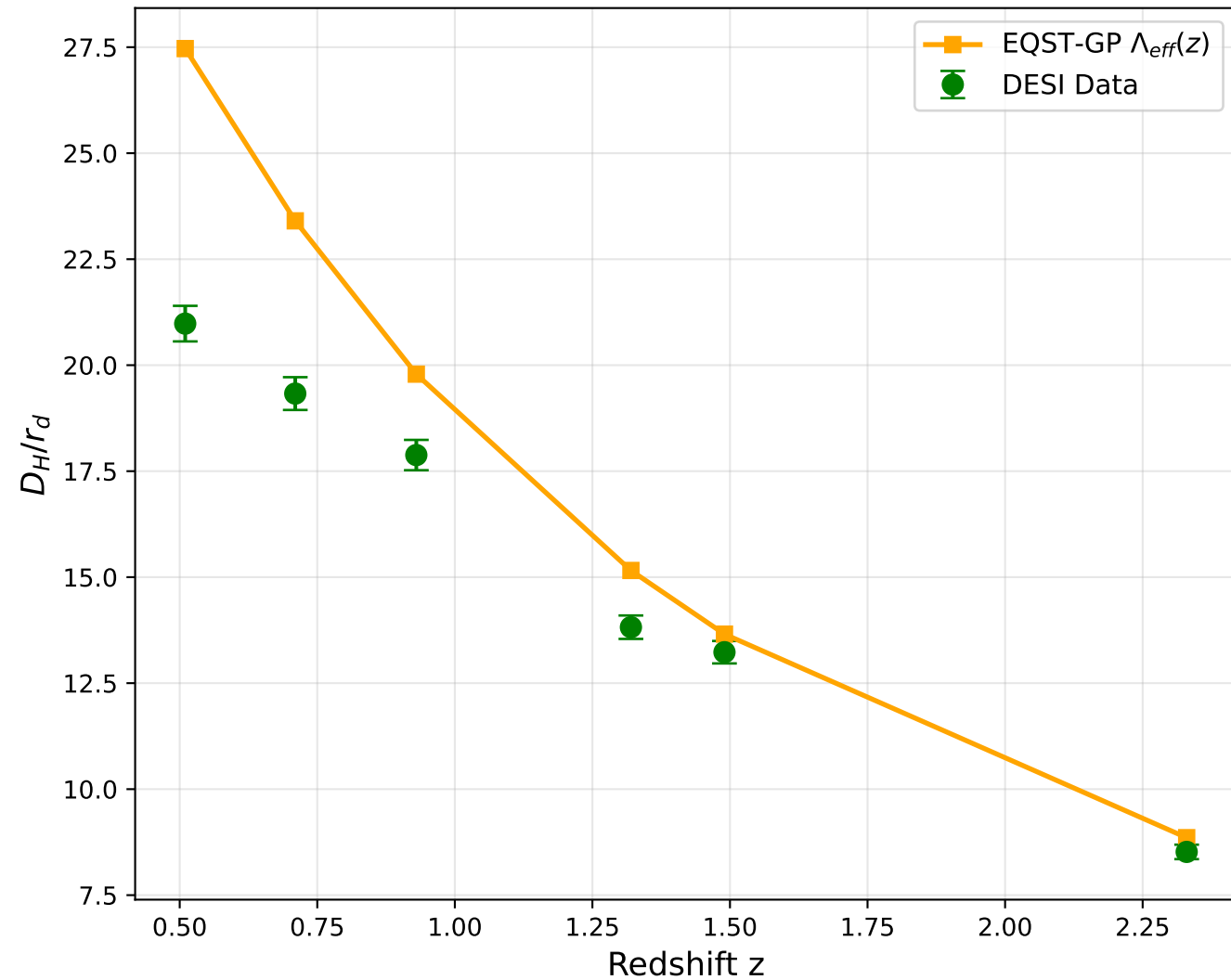
Hubble Distance
