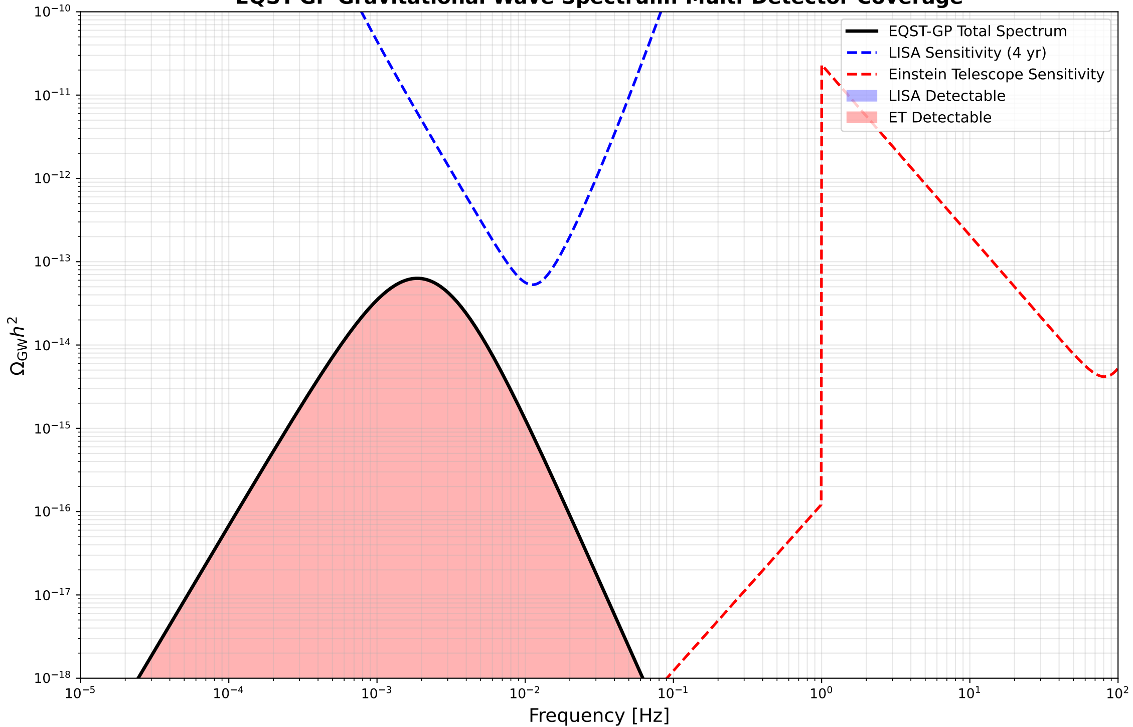
EQST-GP Gravitational Wave Spectrum: Multi-Detector Coverage
