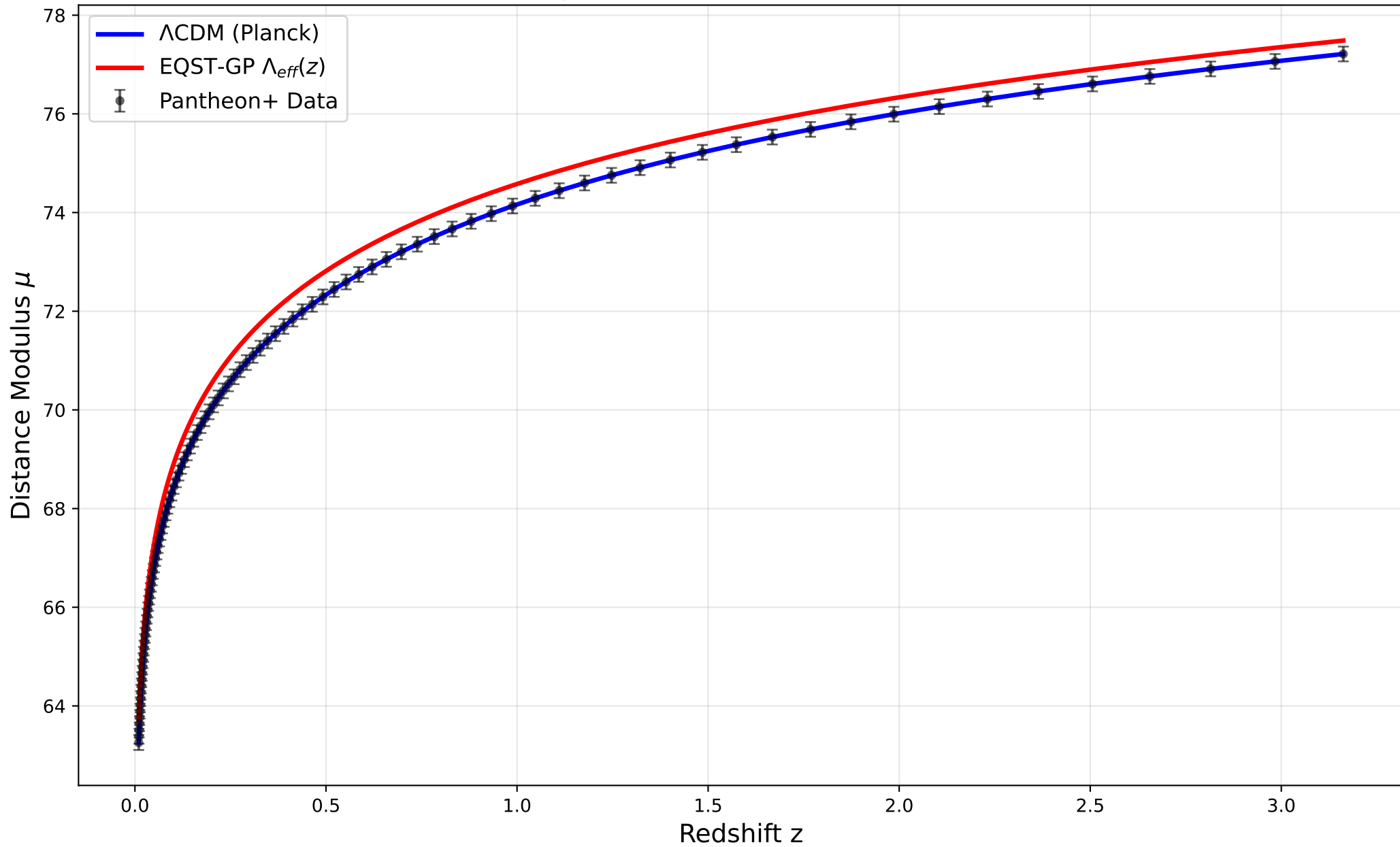
Hubble Diagram: Supernovae Distance Moduli
