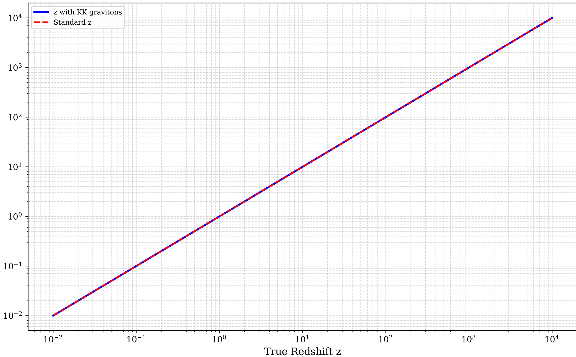
KK Graviton Redshift Correction (m=2.5 TeV)
