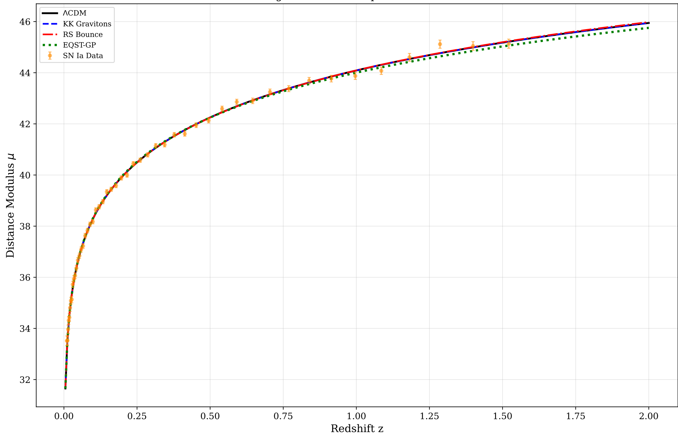
Hubble Diagram: Model Comparison with SN Ia Data
