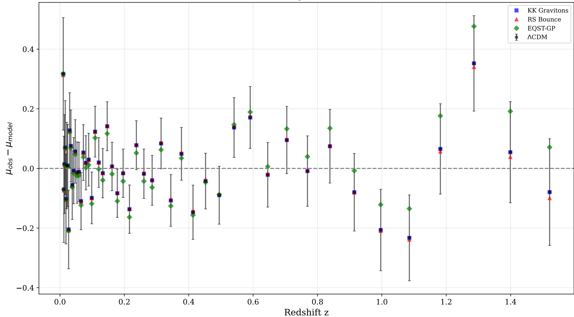
Hubble Diagram Residuals
