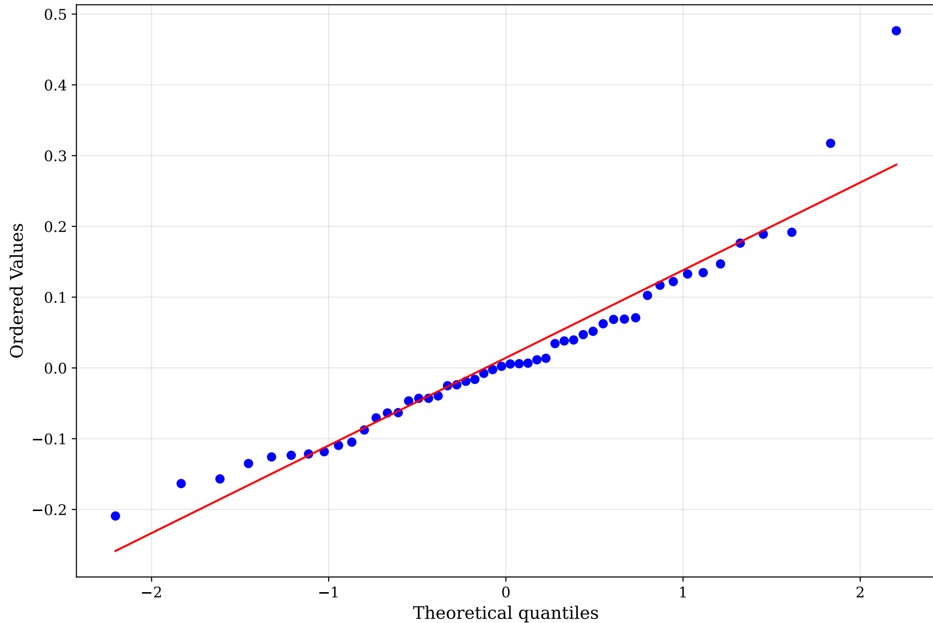
Q-Q Plot: EQST-GP Residuals vs Normal Distribution
