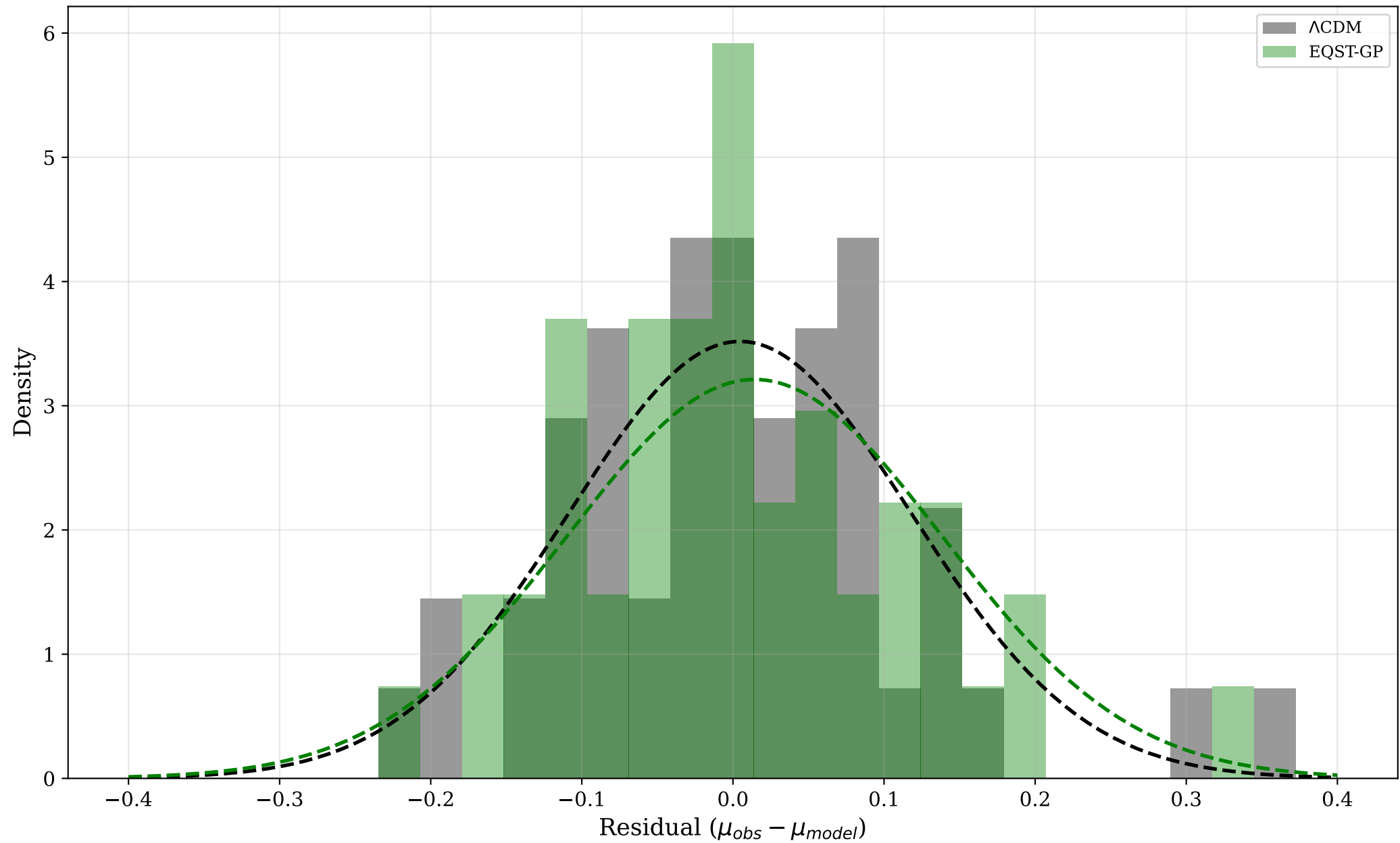
Residual Distributions: LCDM vs EQST-GP
