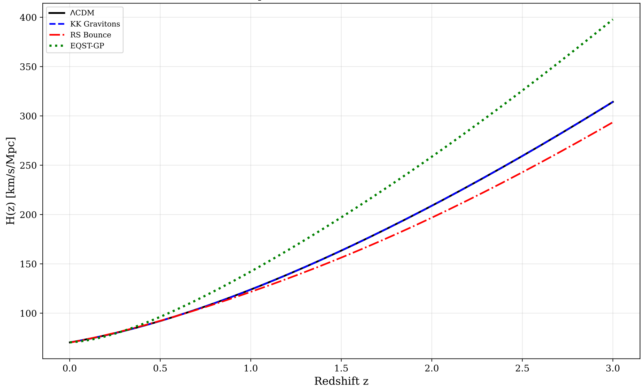
Expansion Rate H(z) Across Models
