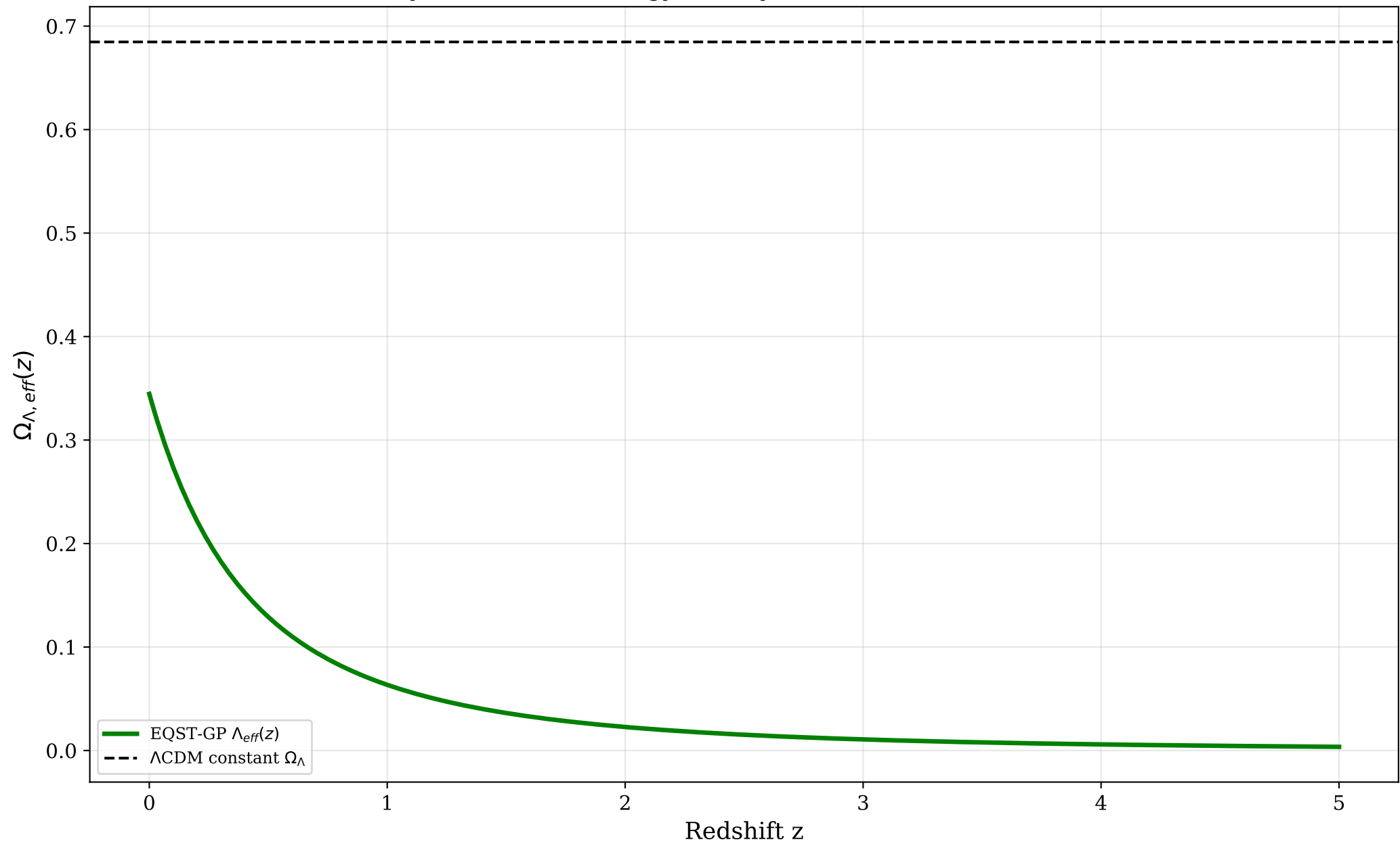
Dynamical Dark Energy Density: EQST-GP \Lambda_{\text{eff}}(z) Evolution
