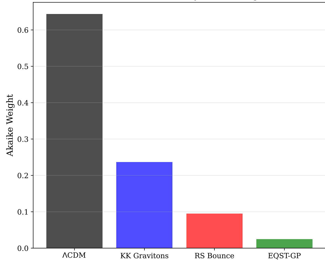
Relative Model Probability (Akaike Weights)
