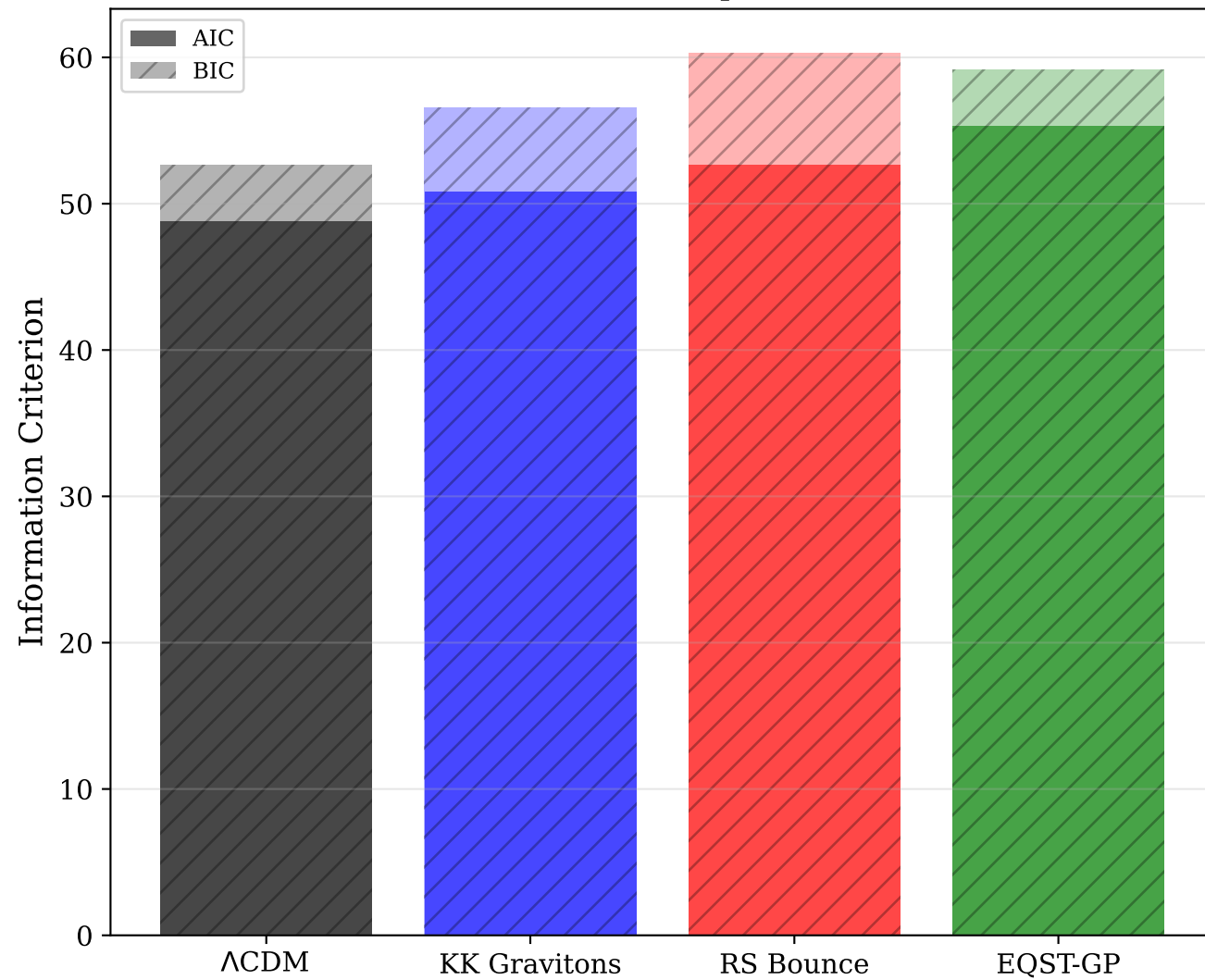
AIC / BIC Comparison
