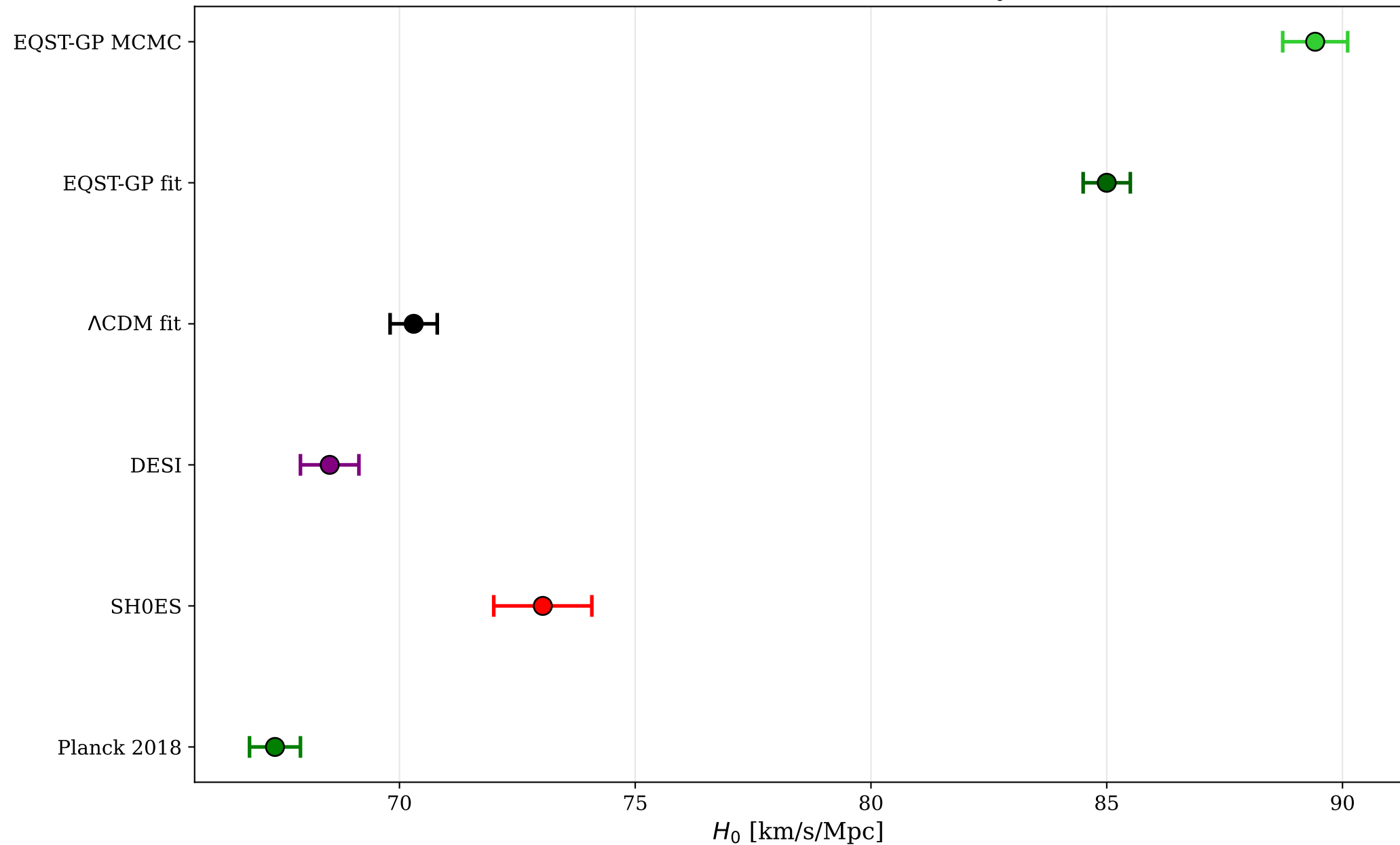
Hubble Constant Tension Summary
