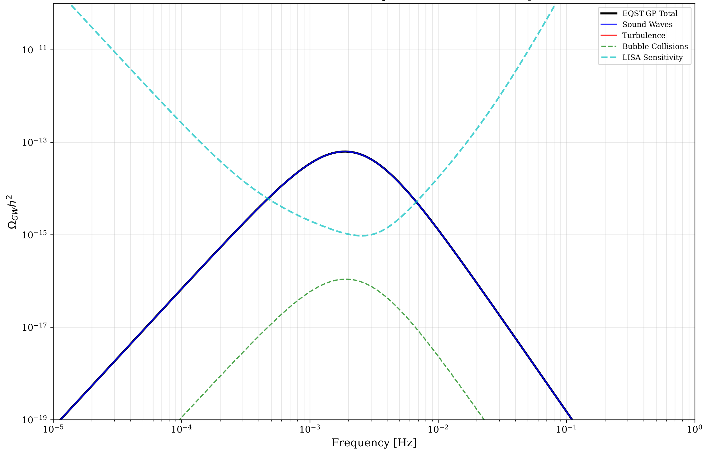
EQST-GP Gravitational Wave Spectrum vs LISA Sensitivity
