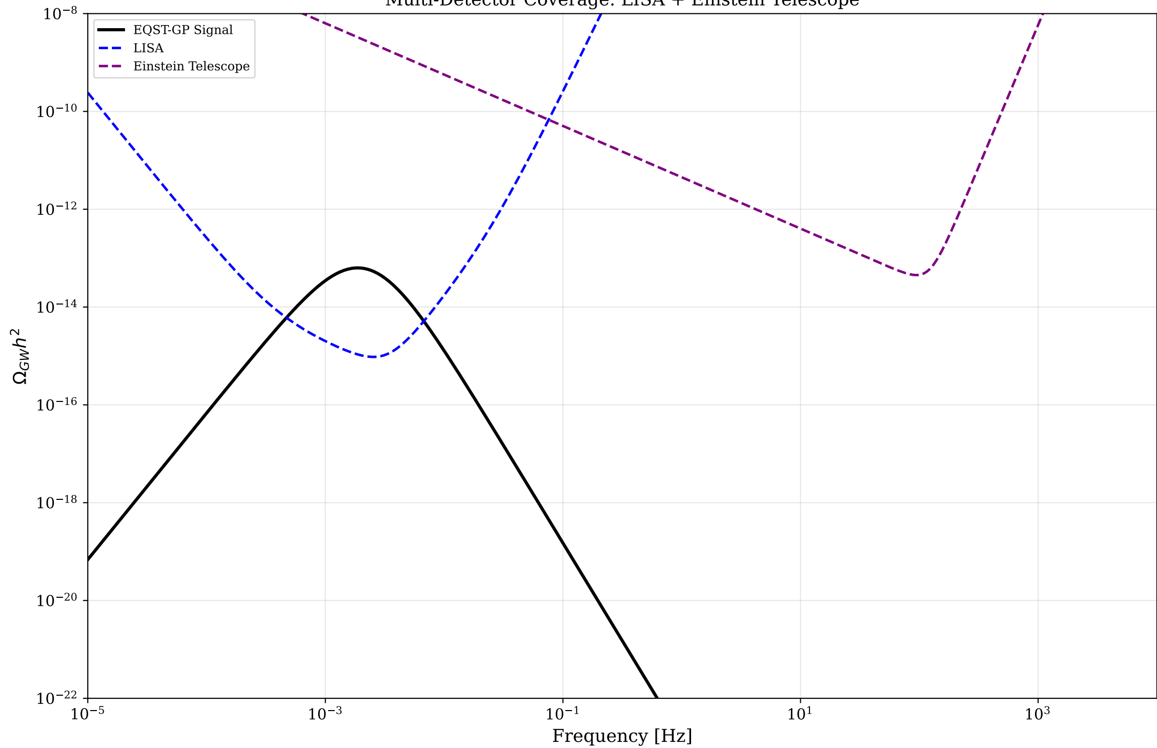
Multi-Detector Coverage: LISA + Einstein Telescope
