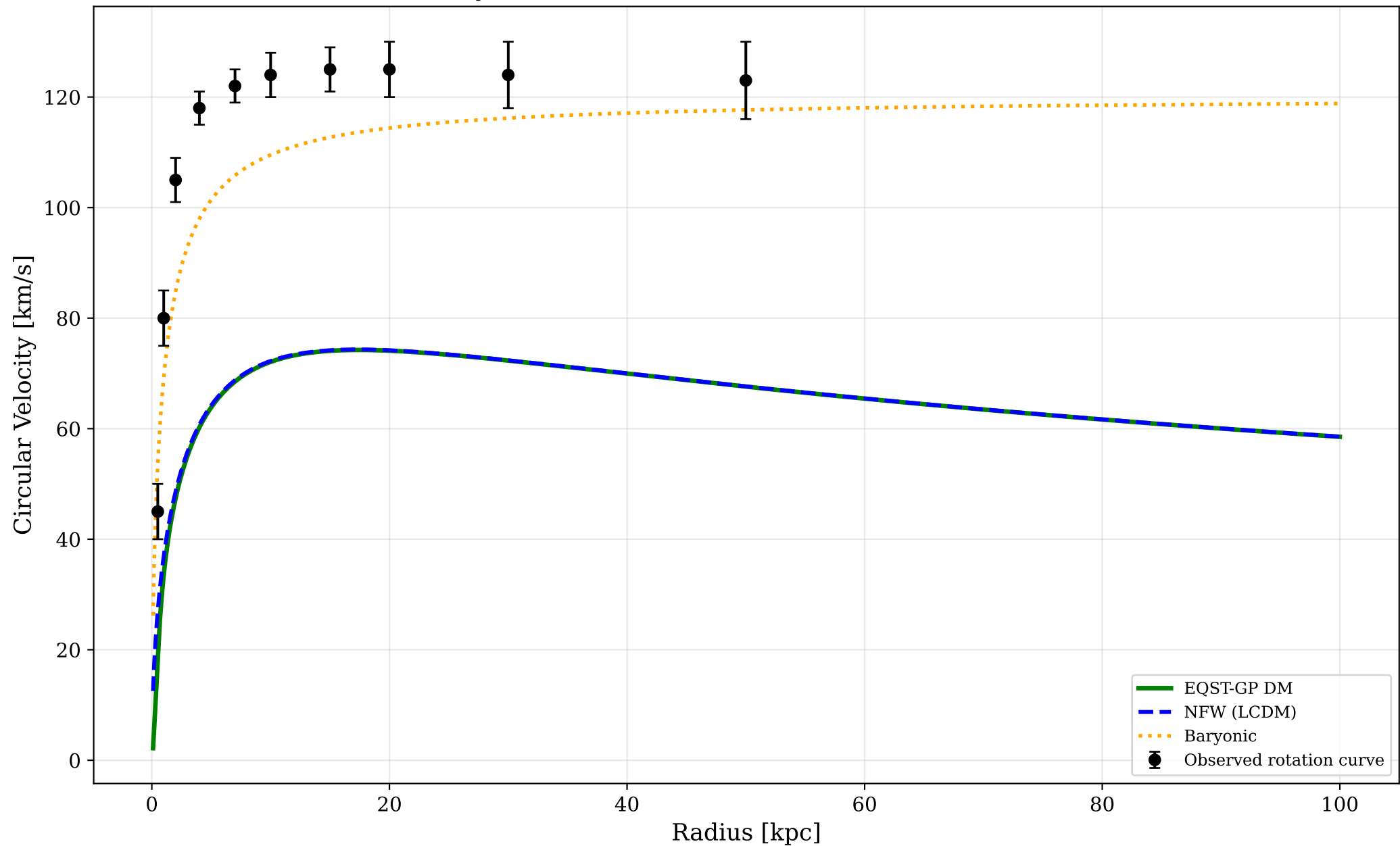
Galaxy Rotation Curve: EQST-GP vs NFW vs Observation
