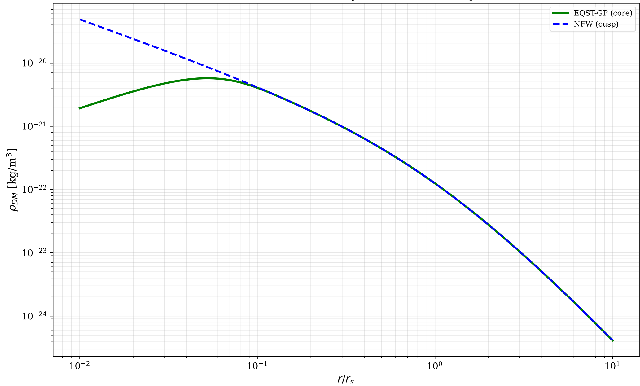
Dark Matter Halo Density Profile: Core vs Cusp
