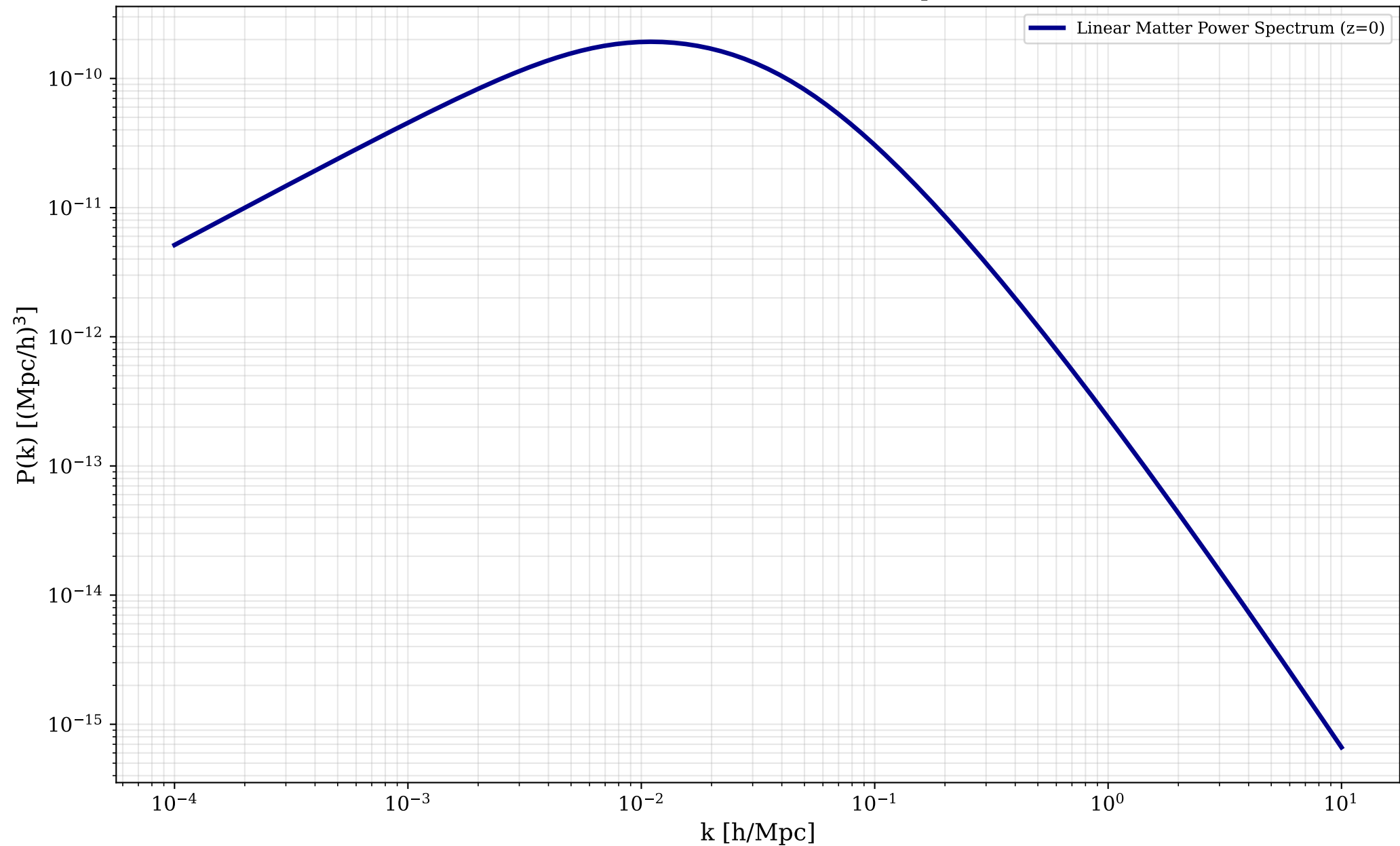
EQST-GP Predicted Matter Power Spectrum
