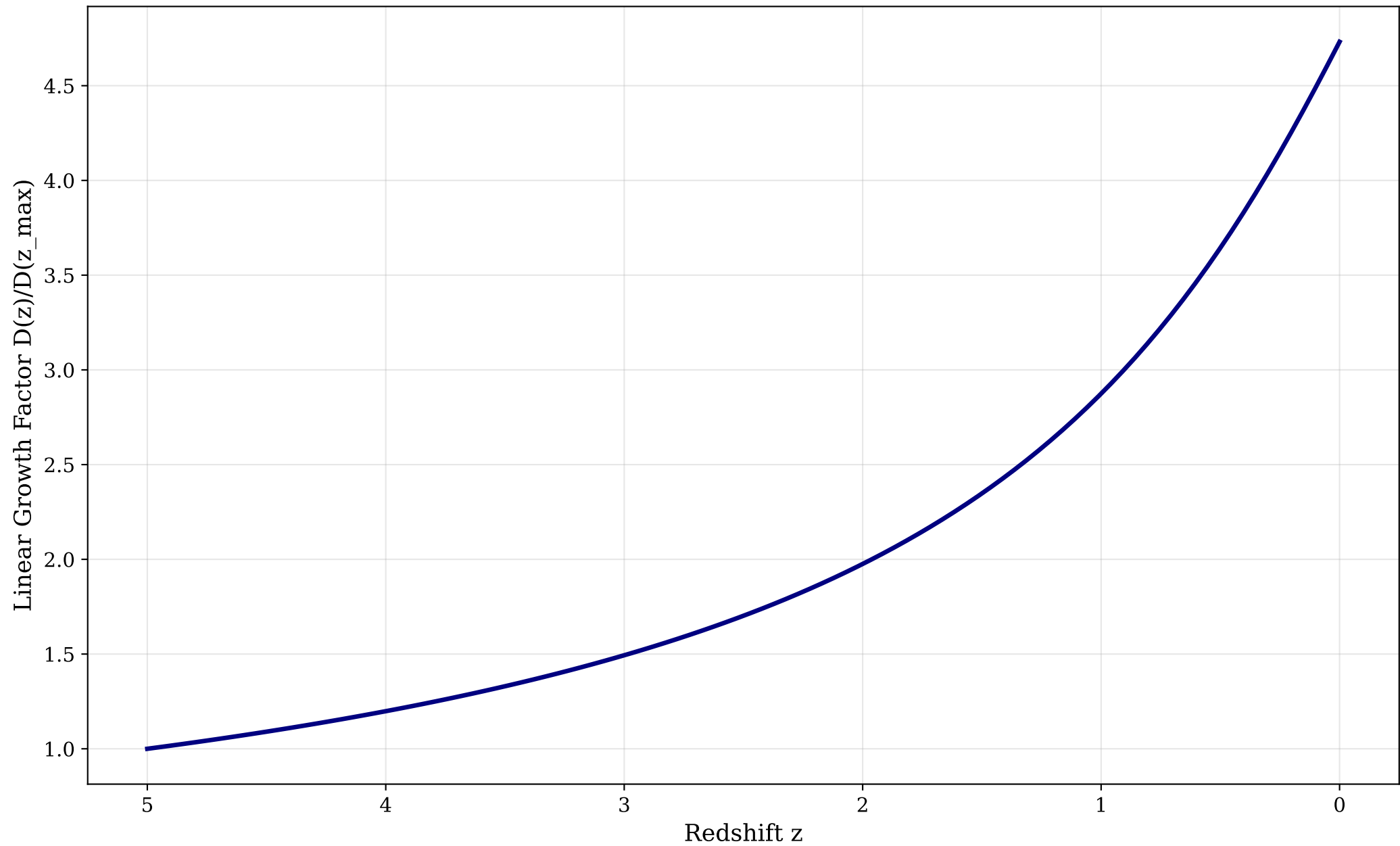
Structure Growth Factor Evolution
