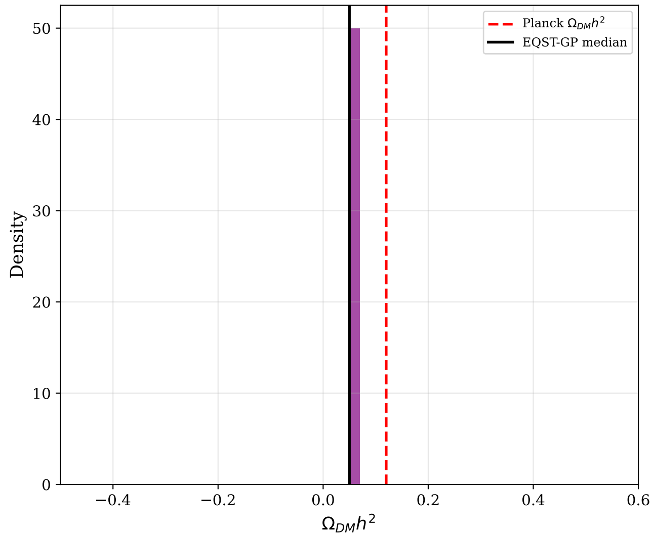
EQST-GP Predicted Dark Matter Relic Abundance
