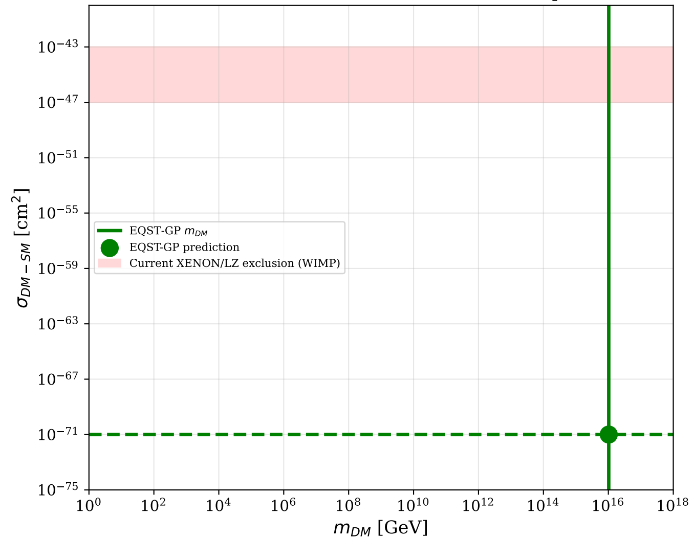
Dark Matter Direct Detection Parameter Space
