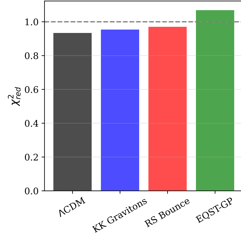
Model Comparison
