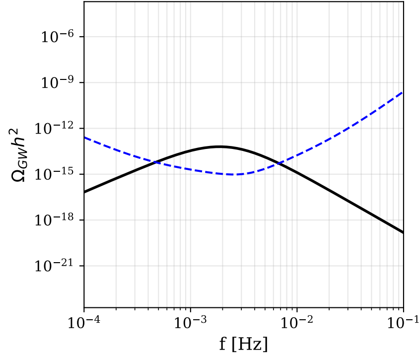
GW Spectrum (LISA band)
