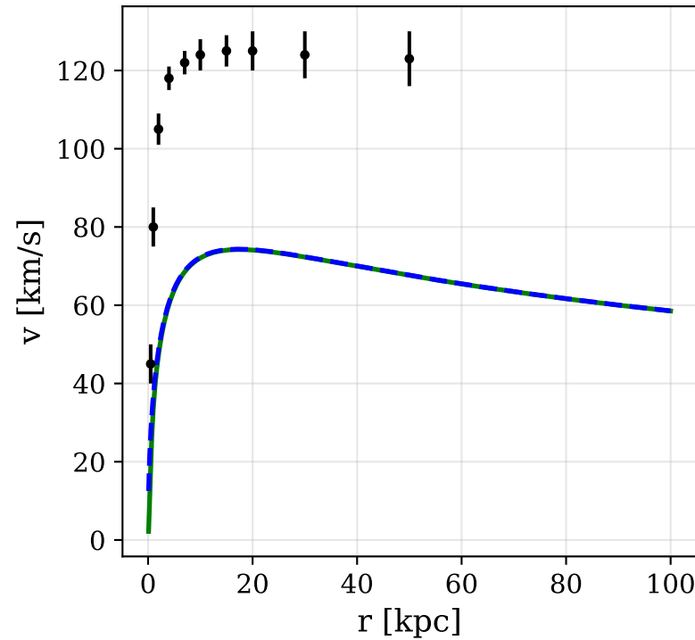
Rotation Curve
