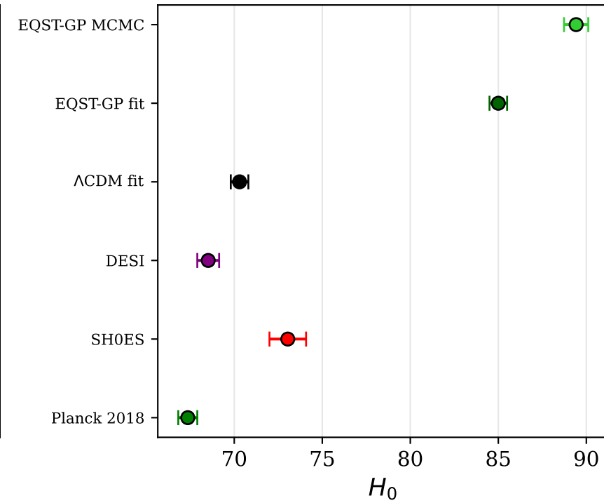
Hubble Tension
