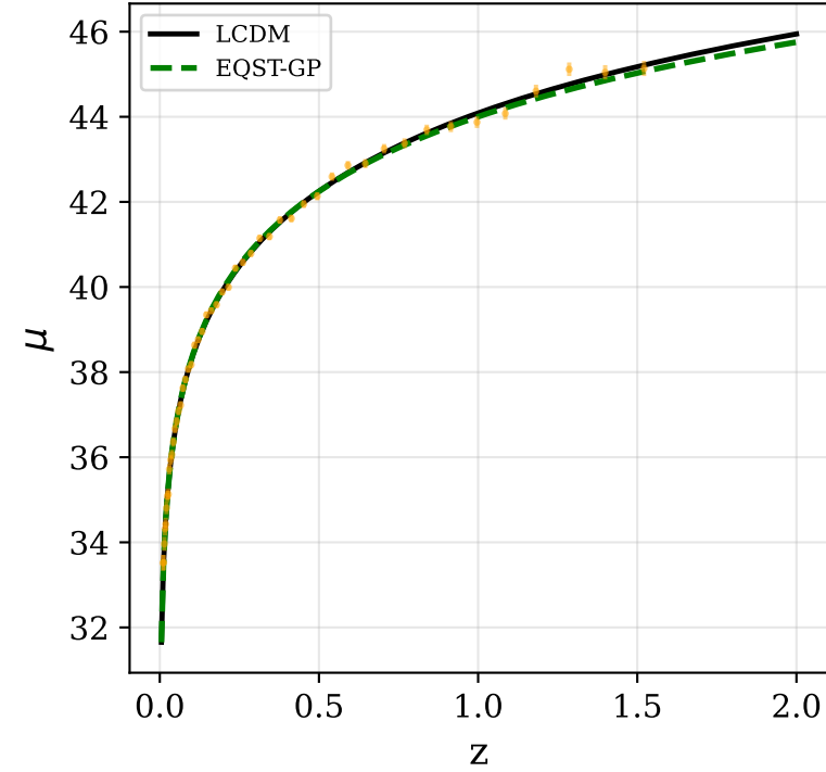
Hubble Diagram
